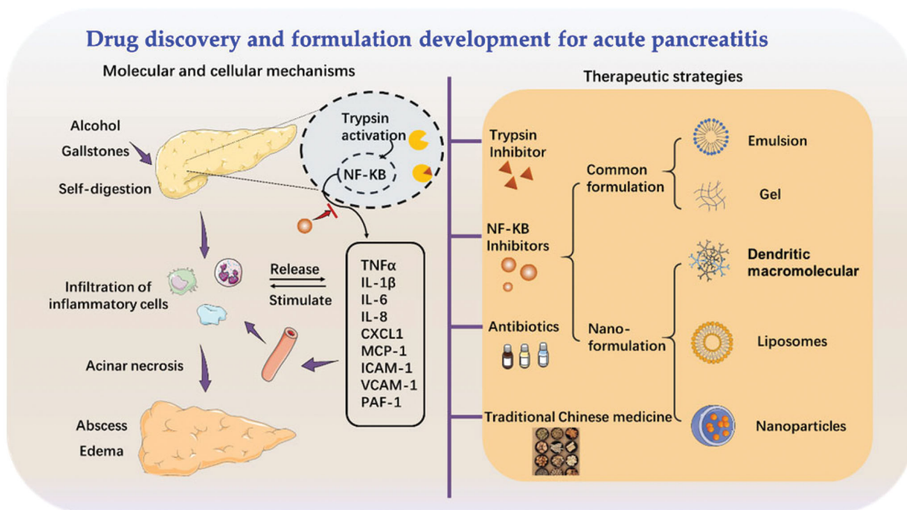
Figure 1. The cellular events in acute pancreatitis and therapy strategies.
