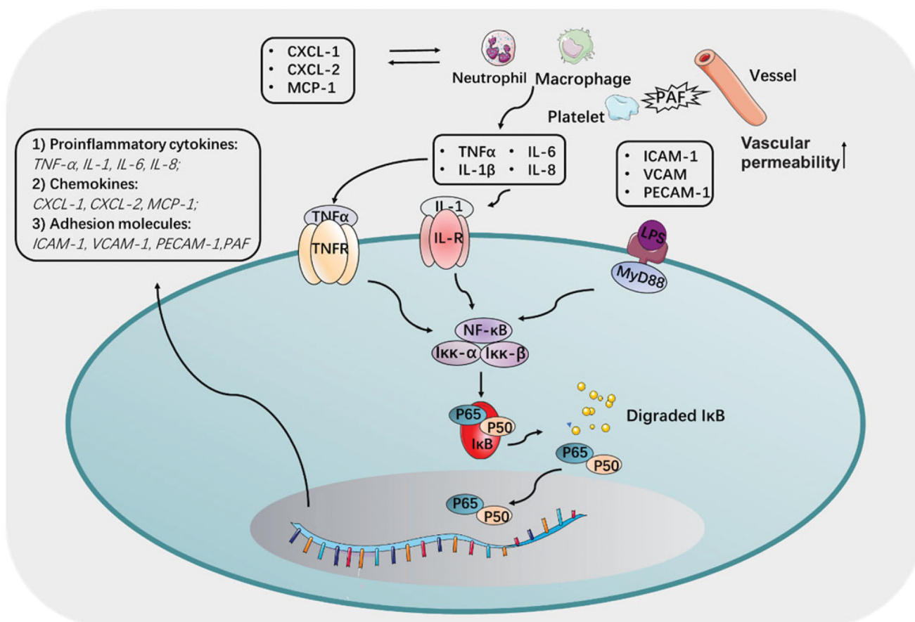
Figure 3. The regulation of NF-κB signaling pathway and involved cytokine and adhesion molecules in acute pancreatitis. Inhibition of NF-κB reduces the induction of pro-inflammatory cytokines, chemokines, and adhesion molecules.
